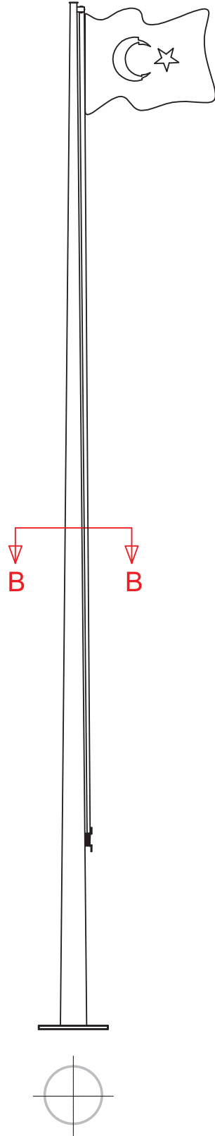
Dairesel Konik Direk - Conical Pole B - B Kesiti - Section B - B
